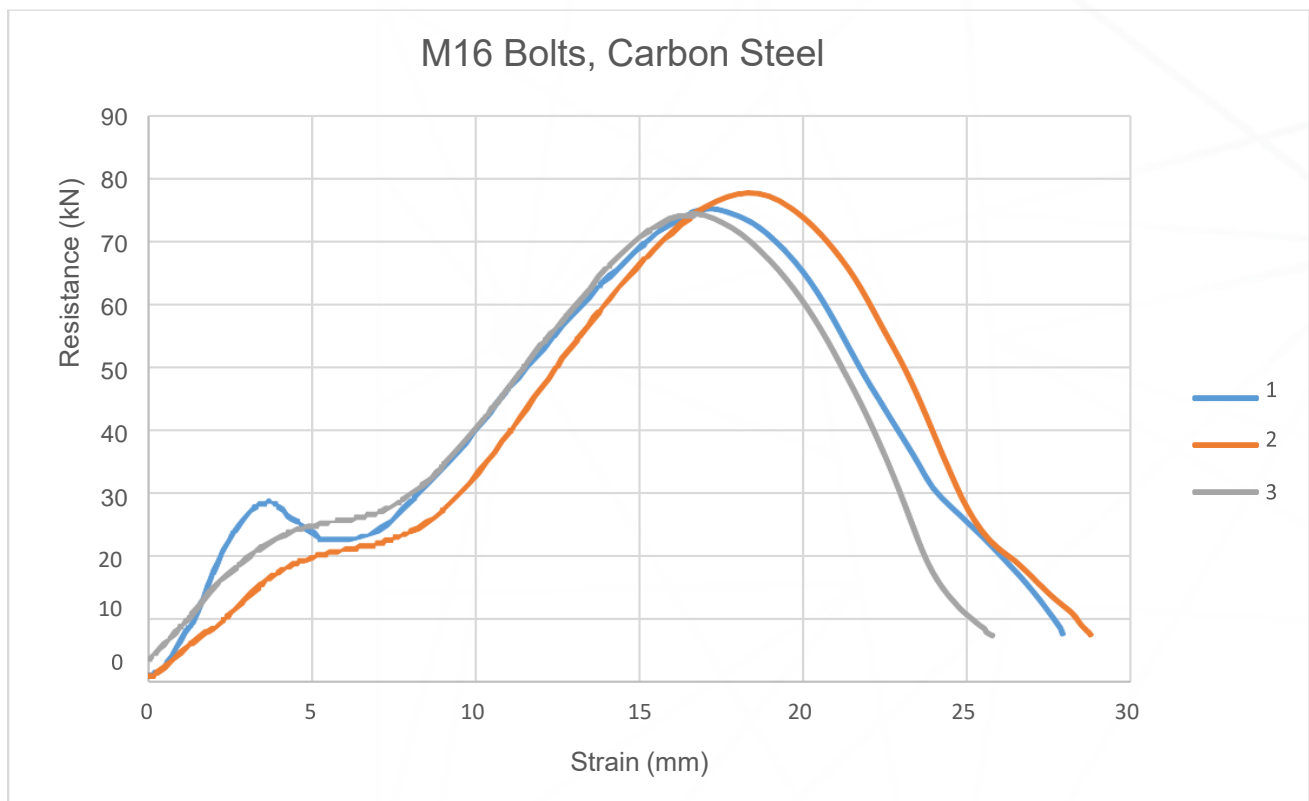
Figure 4. M16 carbon steel test results
