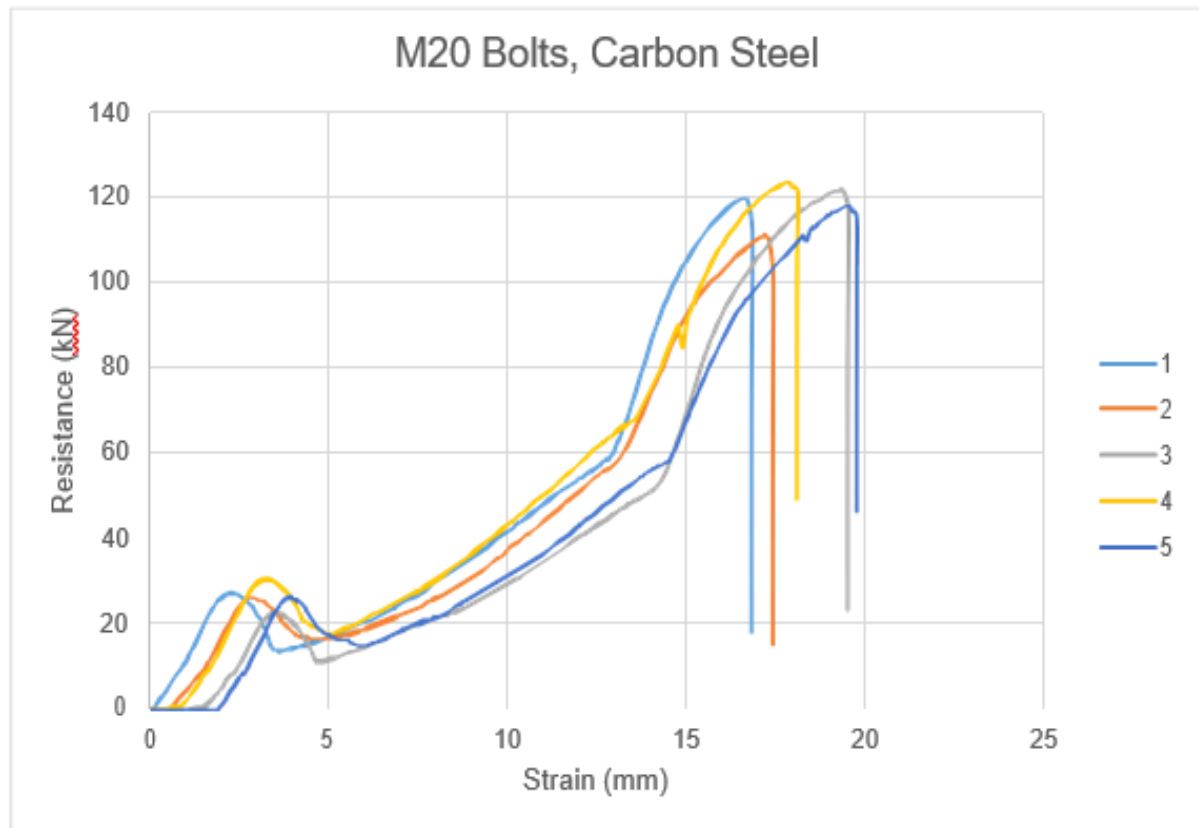
Figure 5. M20 carbon steel test results
