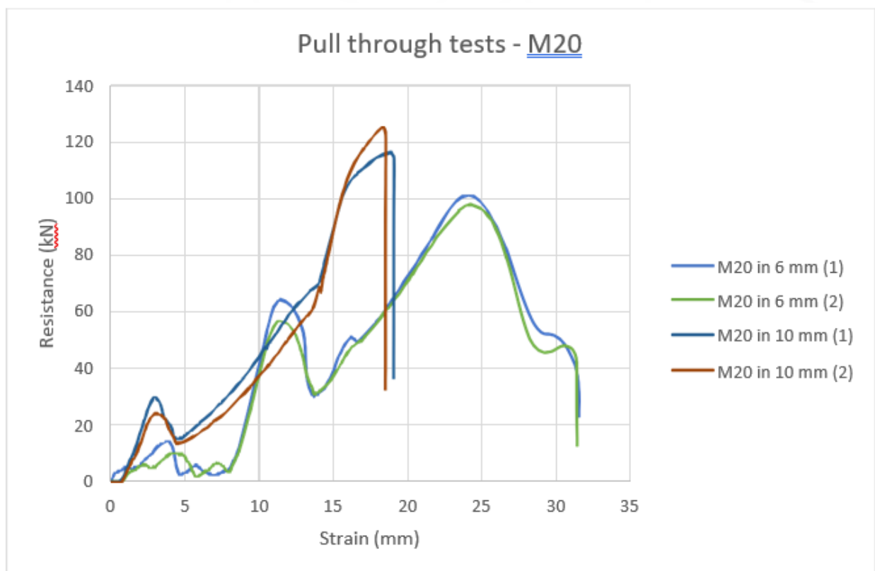
Figure 2. M20 pull-through tests
