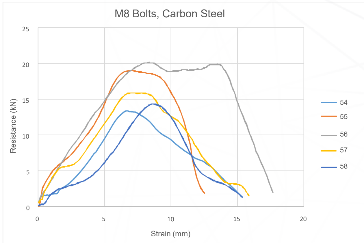
Figure 1. M8 carbon steel test results
