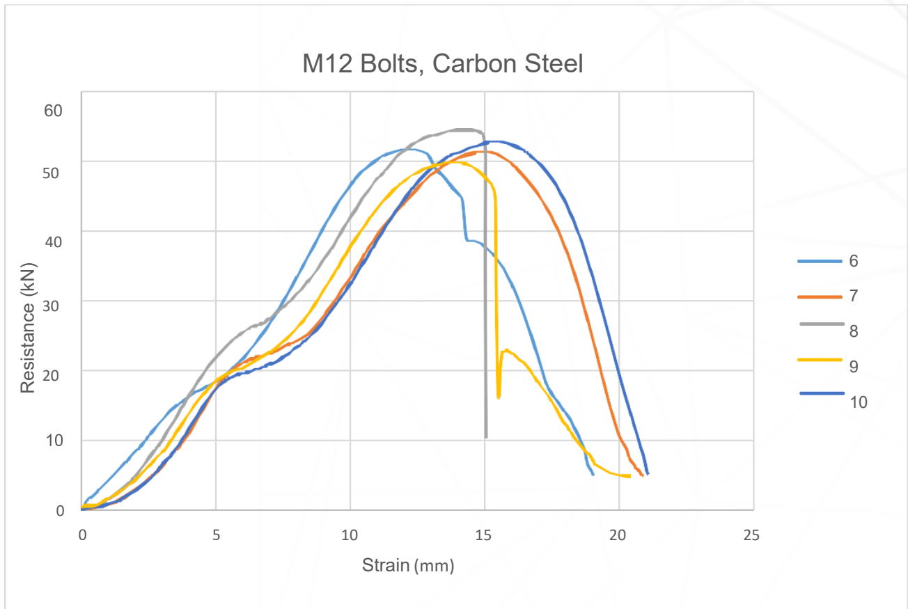
Figure 3. M12 carbon steel test results
