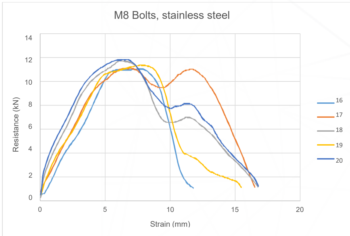
Figure 6. M8 stainless steel test results
