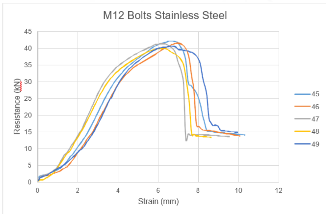
Figure 7. M12 stainless steel test results
