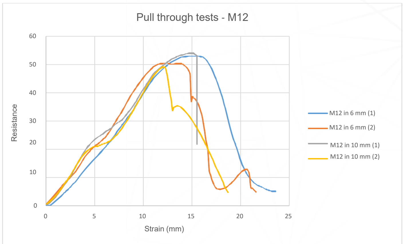
Figure 1. M12 pull-through tests
