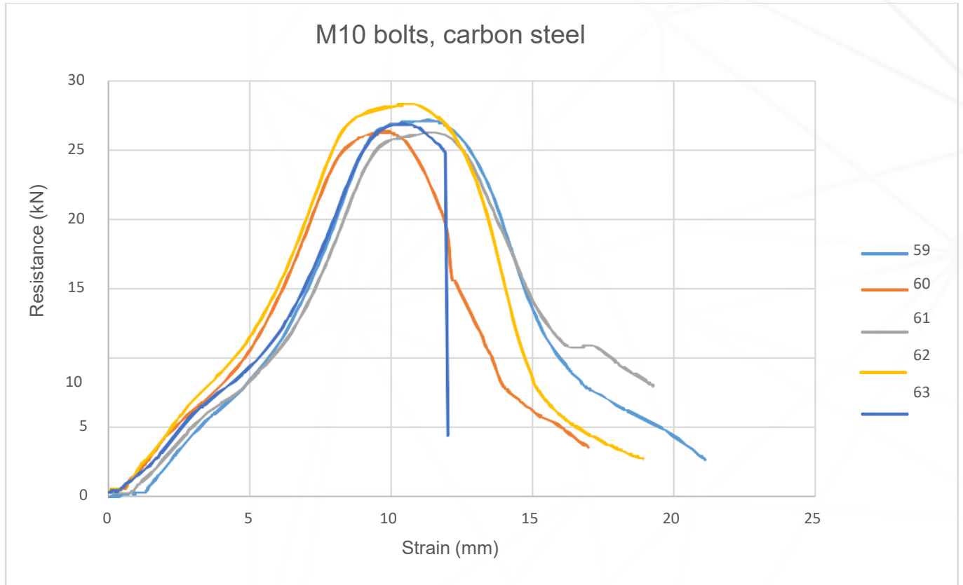
Figure 2. M10 carbon steel test results
